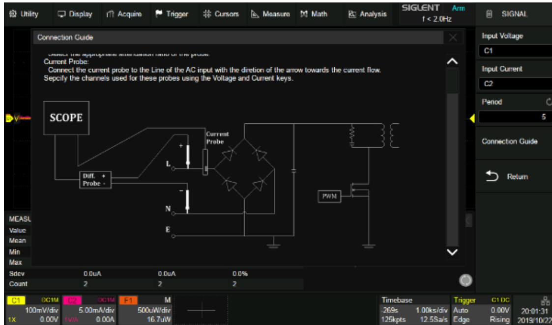
Figure 3: Example of the Connection setup diagram
