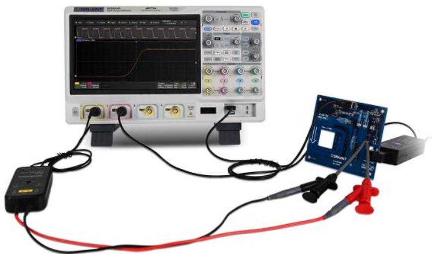
Figure 2: Probe deskew with Siglent DF2001A deskew fixture
