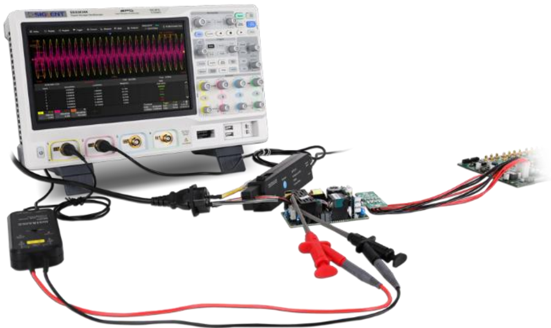
Figure 1: typical test setup for PA
